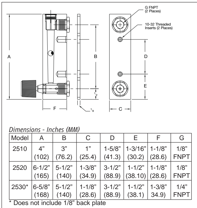
Figure 1 Dimensions - Model 2510, 2520 & 2530
