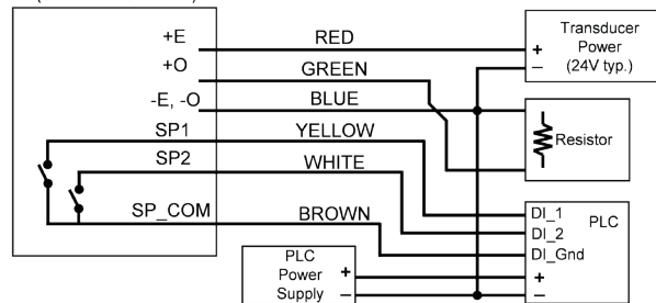
GP, GR: VOLTAGE OUTPUT AND RELAYS (OPEN OR CLOSED)
