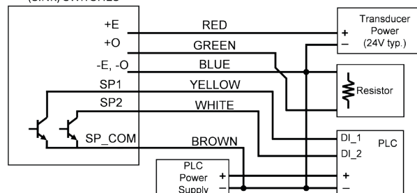
GP, GR: VOLTAGE OUTPUT AND NPN (SINK) SWITCHES
