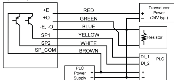
GP, GR: VOLTAGE OUTPUT AND PNP (SOURCE) SWITCHES
