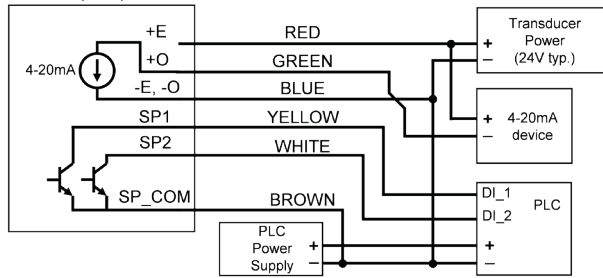
GP, GR: 3-WIRE CURRENT SINK OUTPUT AND NPN (SINK) SWITCHES
