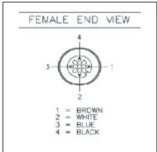
Figure 4-9: M12 Cable Female Connector End view
