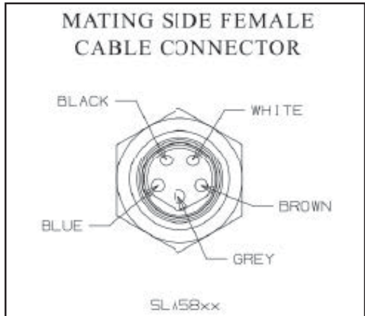
Figure 4-7: M8 Pin Layout
