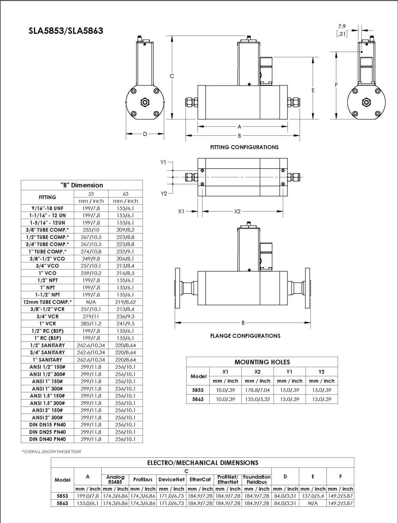
Figure 1-10 SLA5853/SLA5863 Dimensions
