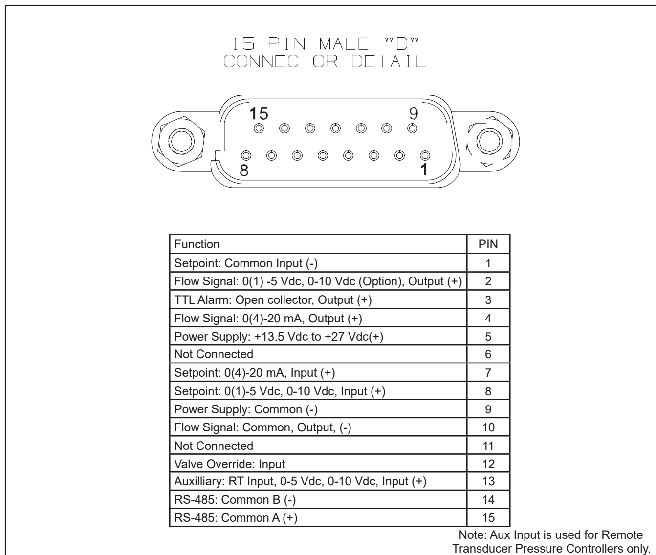
Figure 1-4 SLA5800 Series RS485 15-Pin Analog Connector and Pinouts
