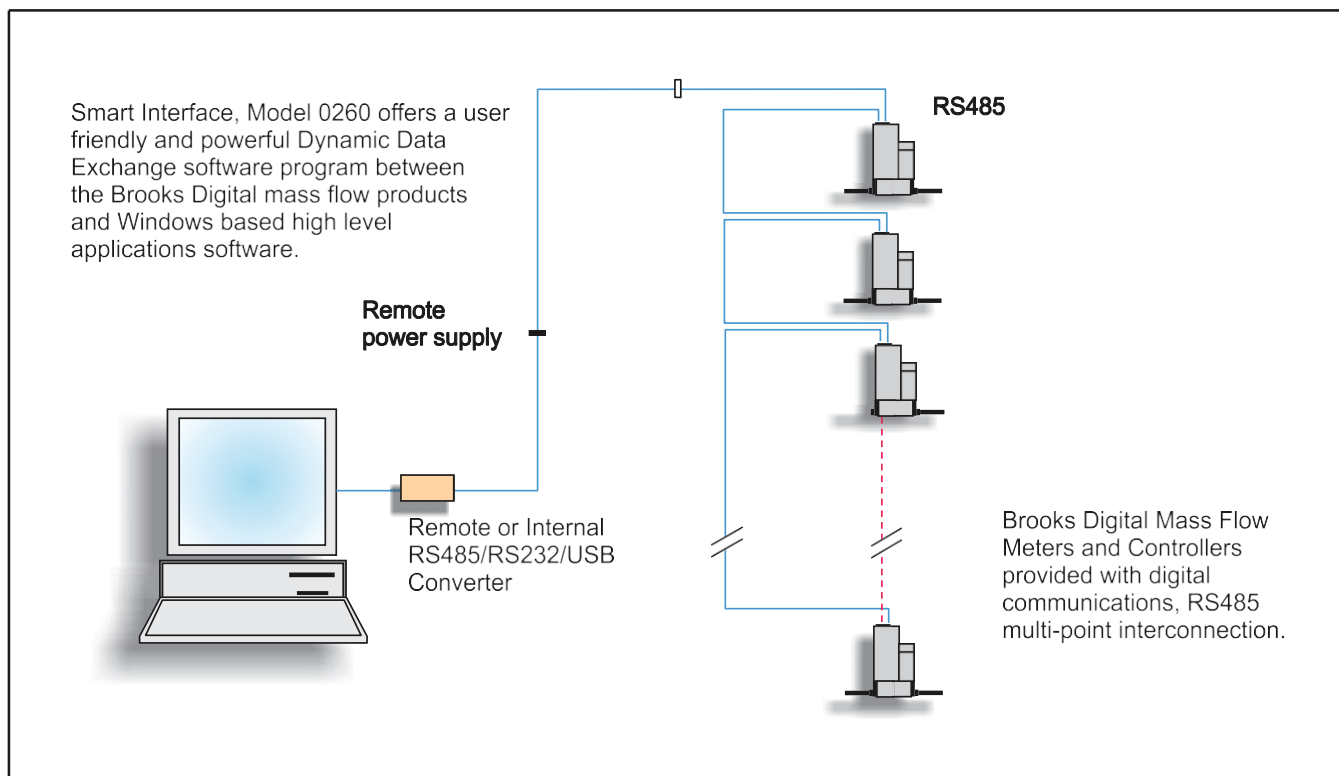
Figure 1-1 General Wiring
