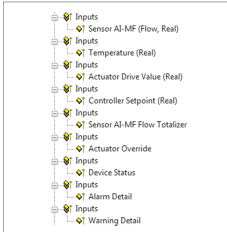
Figure 5-2 Input PDOs
